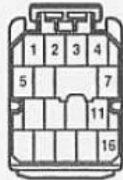
B 16 PIN
