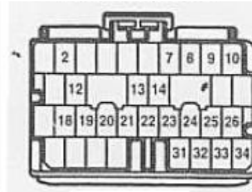
C 34 PIN
