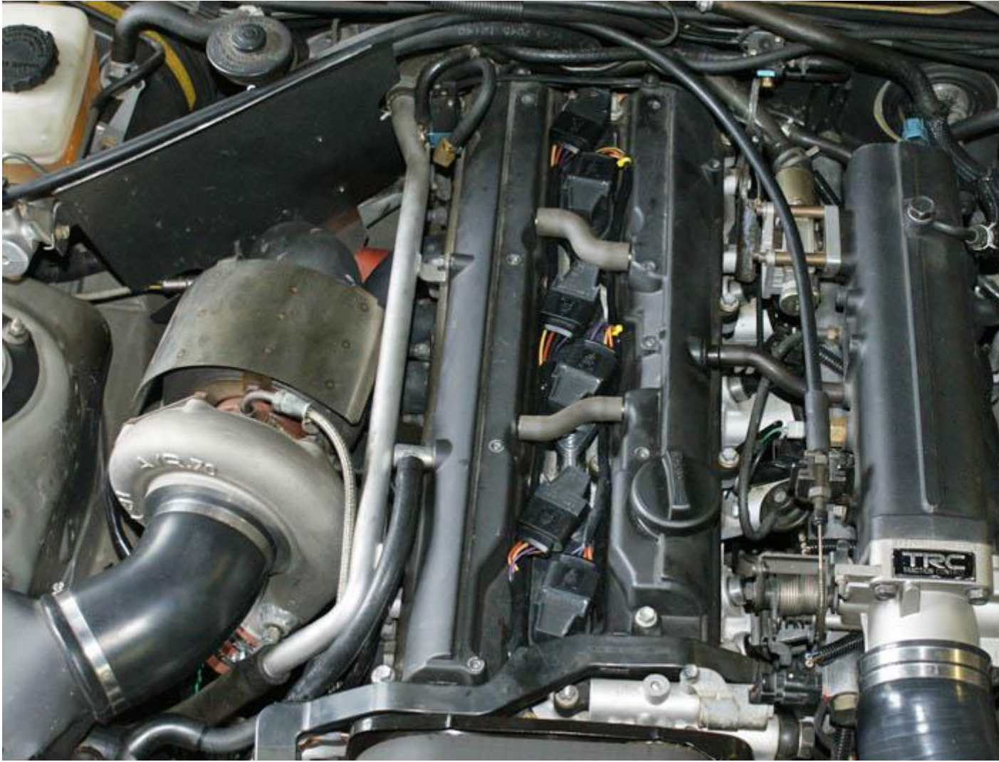
Audi/VW 036905715F Coil on plug coils installed on the 2JZ-GTE
